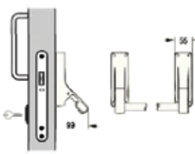
Mortice Panic Nightlatch
